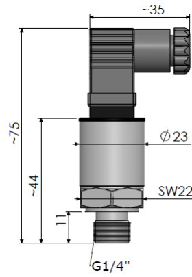
S31: DIN43650-C CONNECTOR
