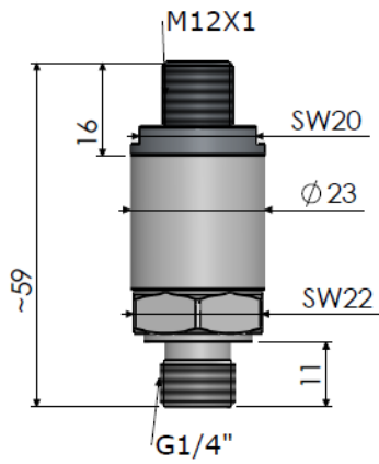
S12/S15: M12 CONNECTOR
